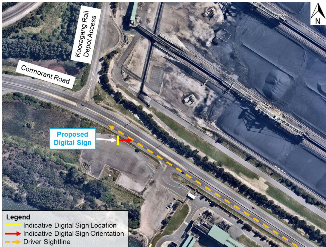
Figure 2.1: Driver Sightlines to the Proposed Digital Sign
