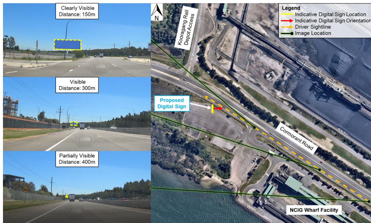
Figure 5.1: In-vehicle sightlines along Cormorant Road westbound
